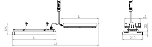
With Emergency Lighting Unit S 0200/0400/0600 TAL
