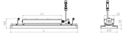
With Emergency Lighting Unit S 0800/1000/1200/1400 TAL
