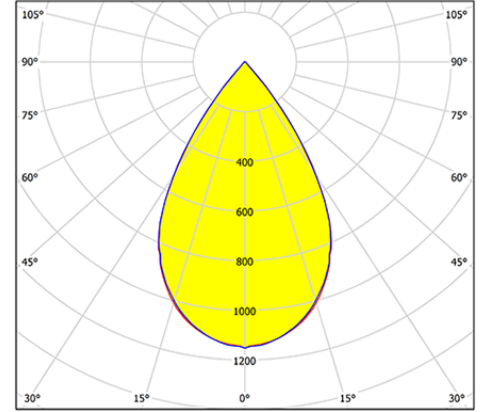
50° - White Reflector
