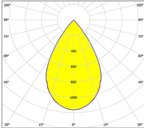
50° - Black Reflector
