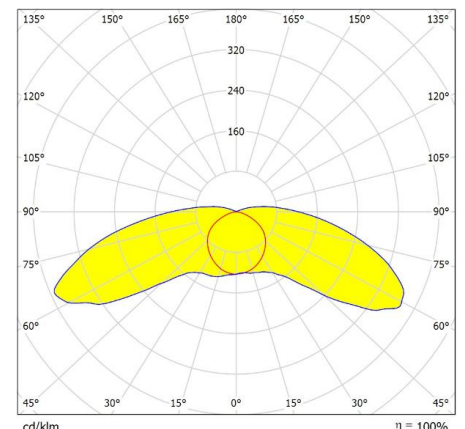
ELUM O.0900.26.40.165° 130°
