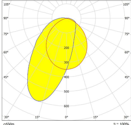
ELUM O.0900.26.40.ASYM
