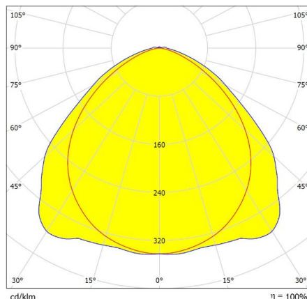
ELUM O.0900.26.40.110° 100°
