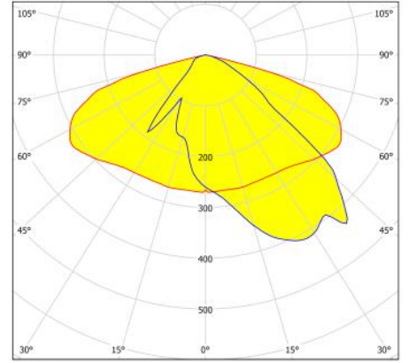
BSLS.0450.250.40.ASL4
