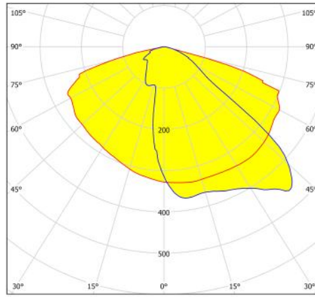
BSTA.550.140.40.L2
