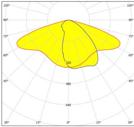
BSTA.550.140.40.L1
