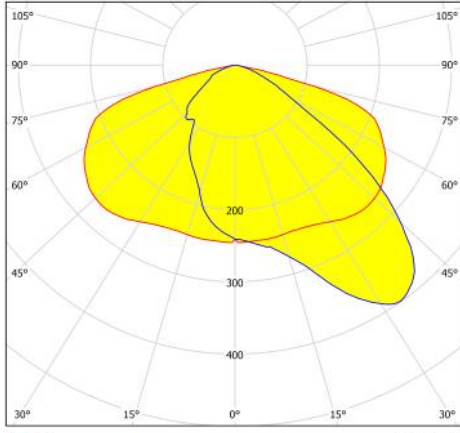
BSTA.550.140.40.L4
